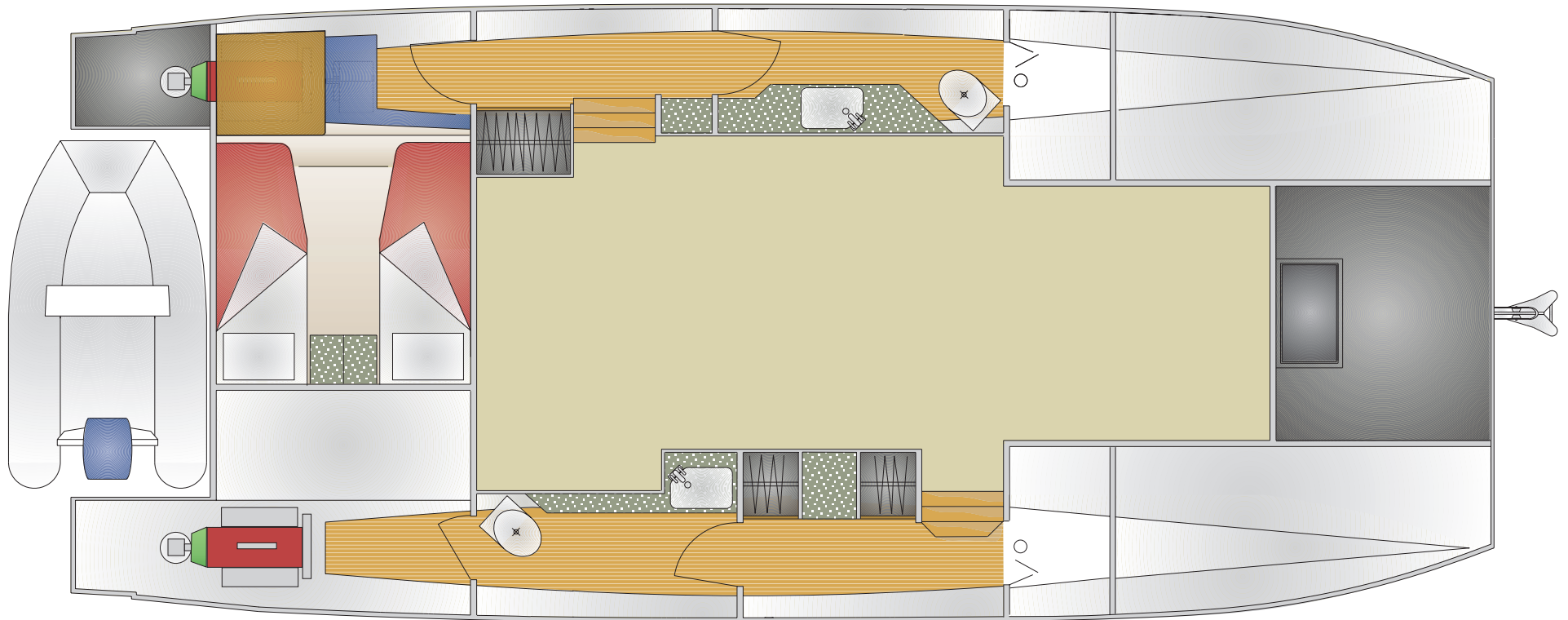
Island Pilot DSe Hybrid — Guest, Heads & Machinery — April, 2008
